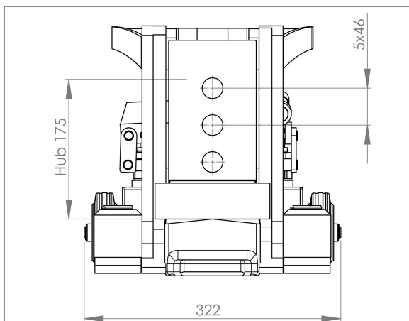
JH 15 G plus | Art.No. 01 150 102-G | Frontansicht | Front view
