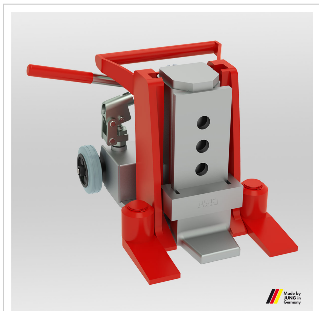
JH 15 G plus | Art.No. 01 150 102-G | Frontansicht | Front view
